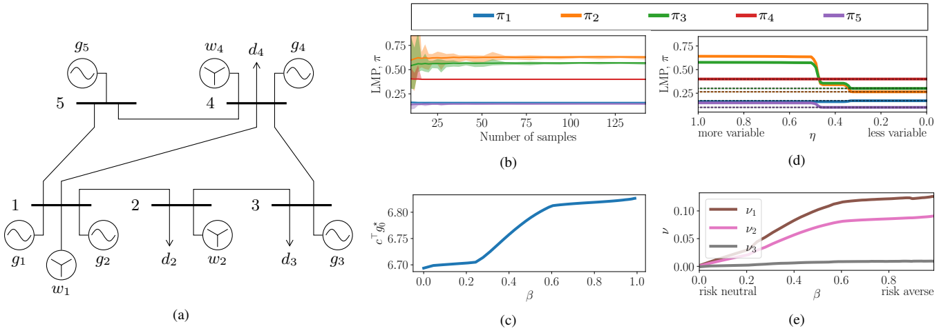
Fig. 1. Evaluation of the prices for the 5-bus network in (a), depicting the (b) mean and range as a function of sample complexity with \gamma = \beta = 0.9 , (c) nominal cost of generation as a function of \beta with \gamma = 0.6 , (d) effect of scaling forecast error by \eta for \gamma = \beta = 0.6 , where the dashed line shows the LMP of the nominal ED, and (e) reserve price, \nu , as a function of \beta with \gamma = 0.6 .
